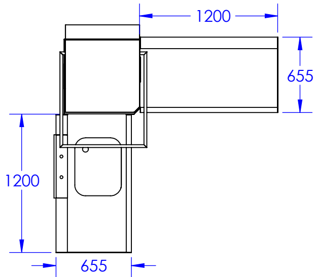
Plan View
